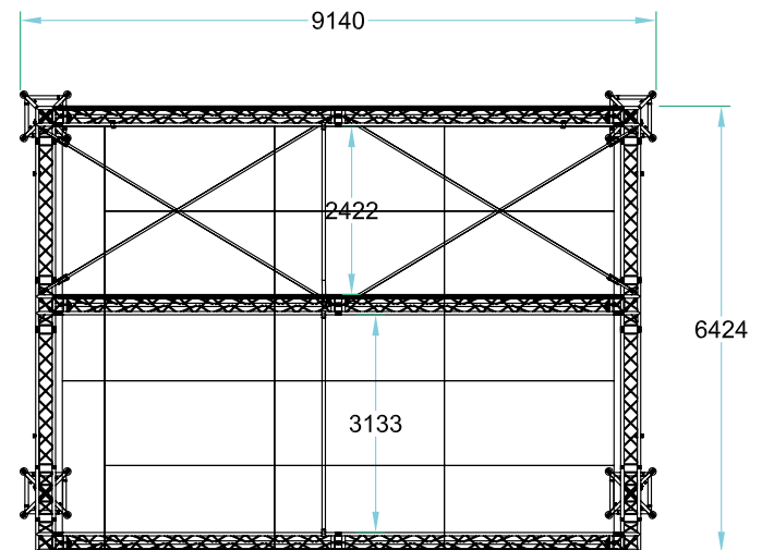
Plan View
